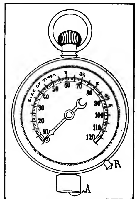
Fig. 3—Schubert tire gauge
